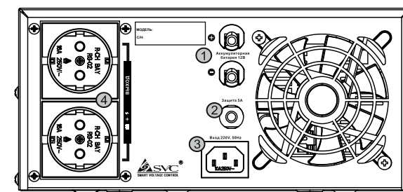
DIL-600/DIL-800/DIL-1000
